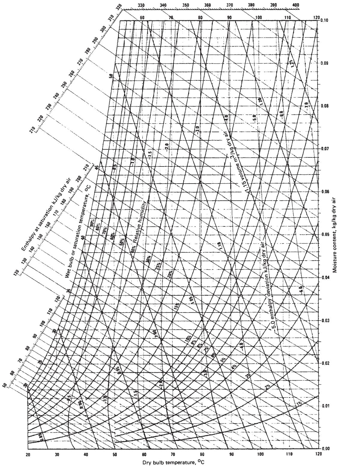
FIG. 12-36 Psychrometric chart: properties of air and water-vapor mixtures from 20 to 120°C. (Carrier Corp.)
